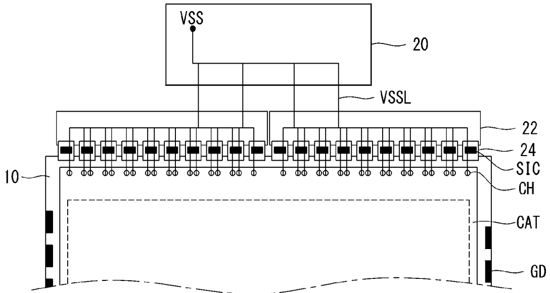
FIG. 1 (RELATED ART)
